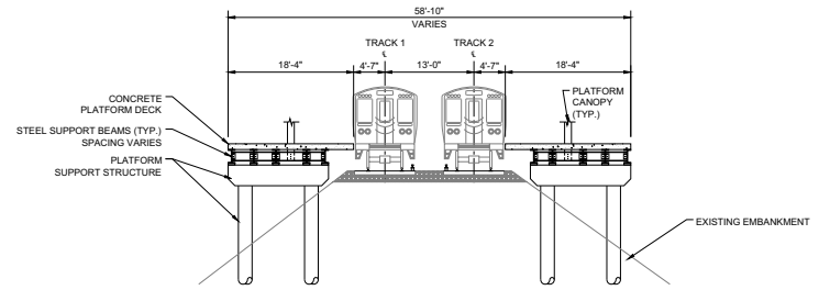
Typical Section - 2 Track Structure along the Purple Line
