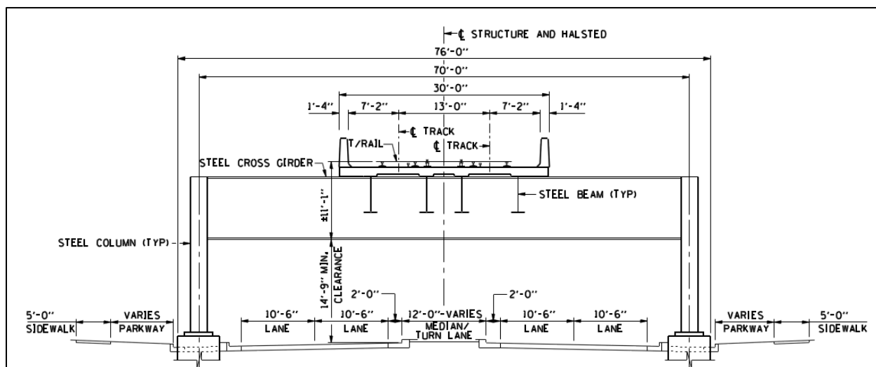
Figure 2-6: Typical Straddle Bent Cross-Section for Halsted Rail Alternative
