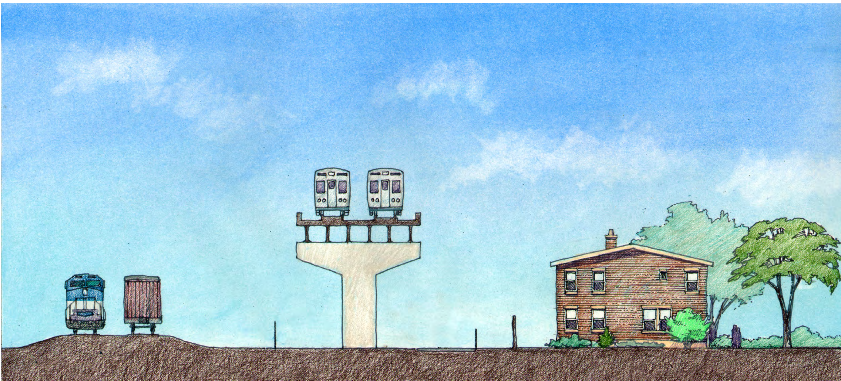
East Side Option typical cross section (looking north)
