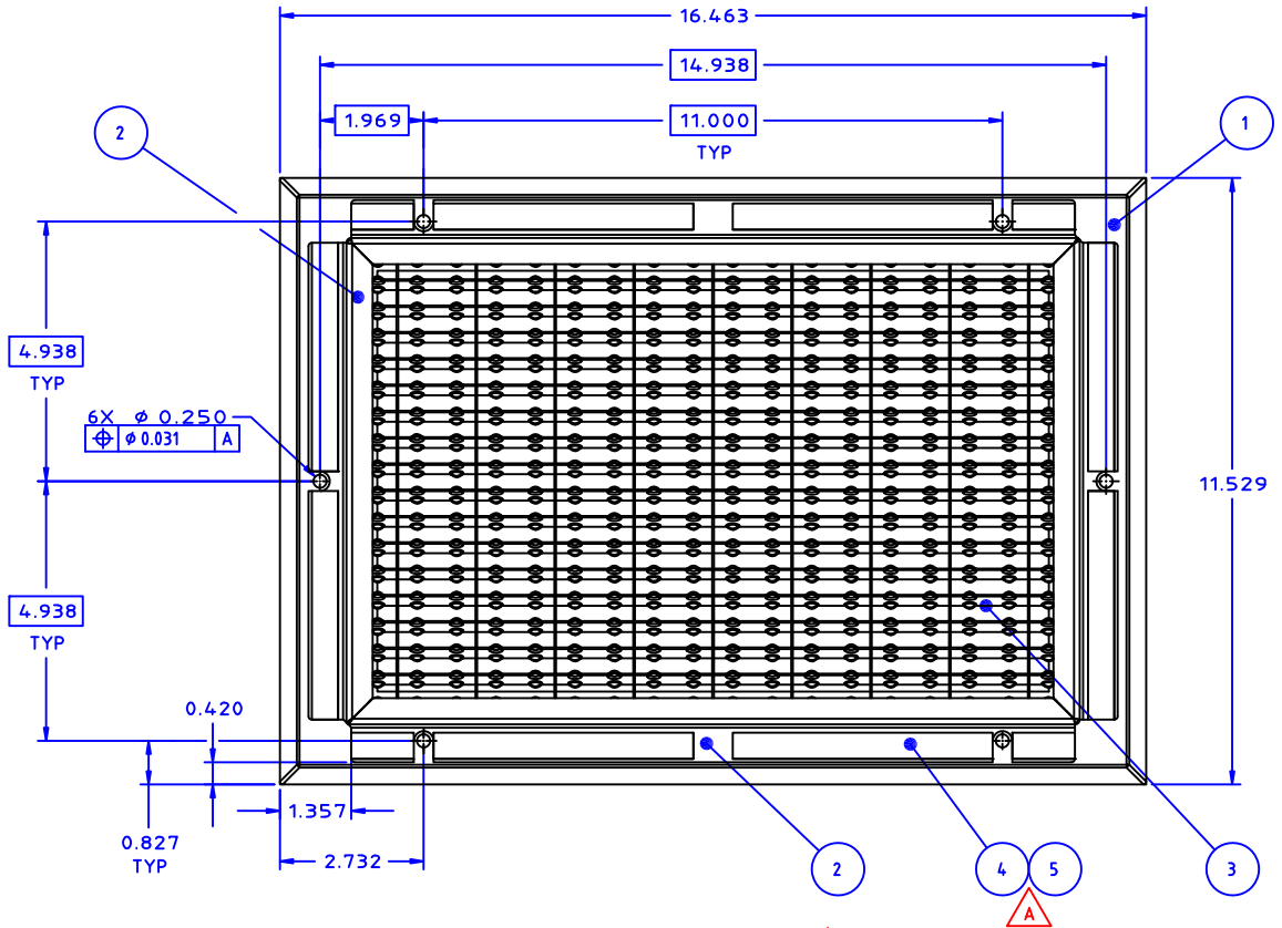
VIEW A1
