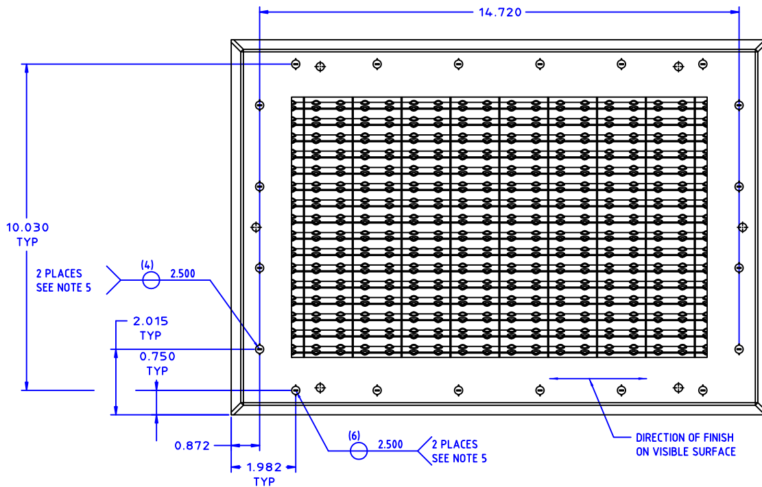
VIEW B1
