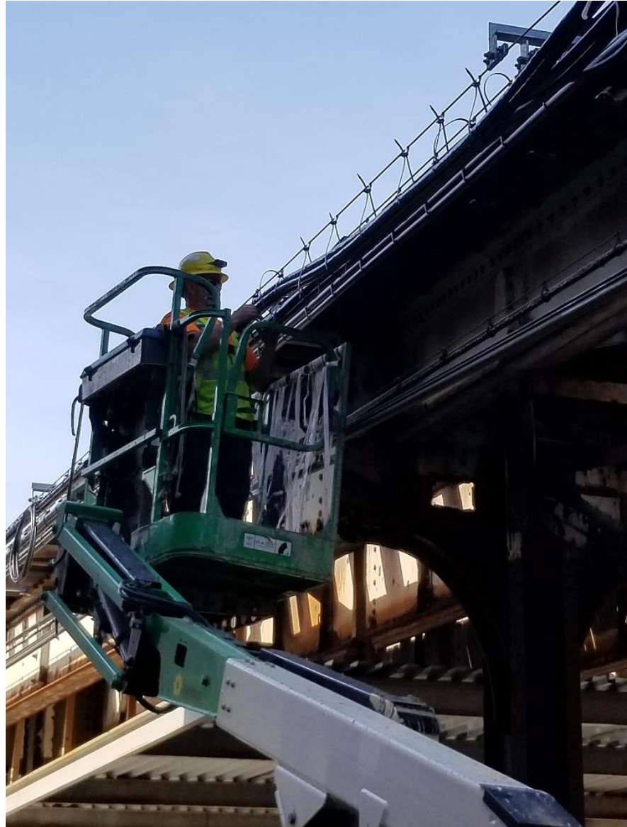
Securing Newly Pulled Signal Cables
